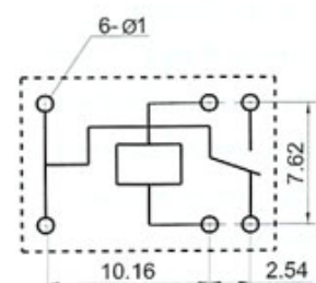
Wiring Diagram & PCB layout
