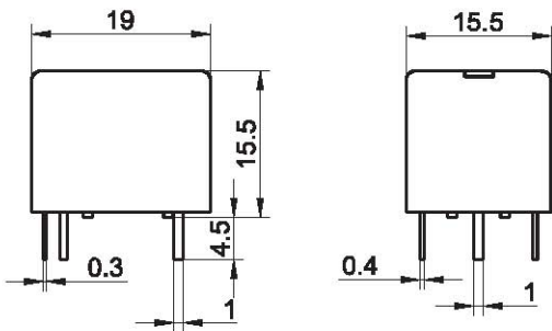
Outline Dimensions
